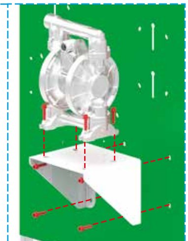
Holes for bracket P/N 33591 for diaphragm pumps 1/2" e 1" S. 120-PPB e S. 1000-AB
