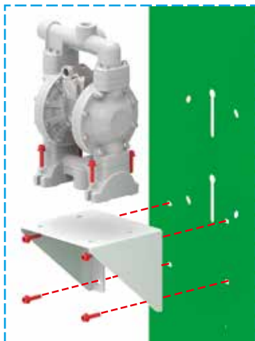
Holes for bracket P/N 33590 for diaphragm pumps 1/2" S. 120-AB, S. 120-PPAB e S. 120-PPB
