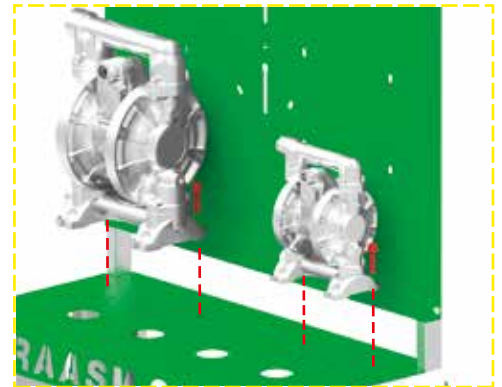
Holes for diaphragm pumps 1" S. 1000-AB
